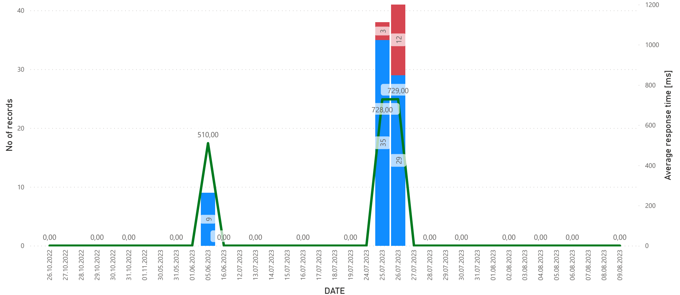
No of Payment Initiation Request and Errors per Day
